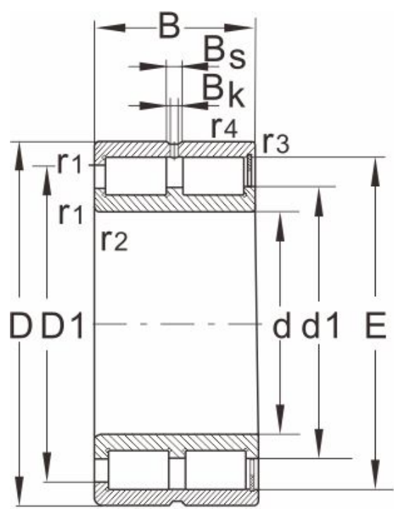
NNCF
